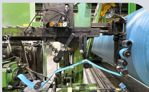
Production of rubber belts
